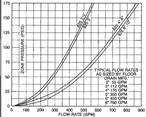
RELIEF VALVE DISCHARGE RATES for 825 Reduced Pressure Devices
